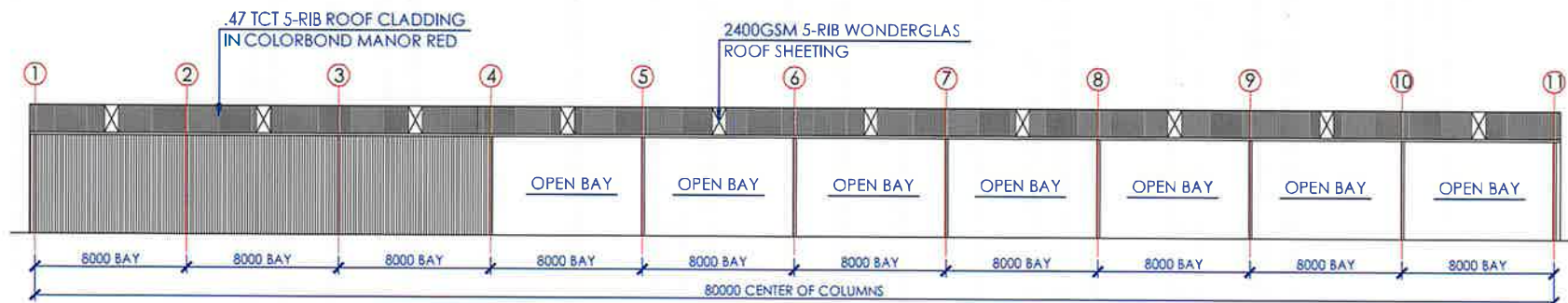
EAST ELEVATION
