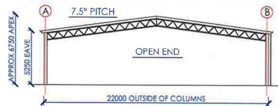
NORTH ELEVATION
