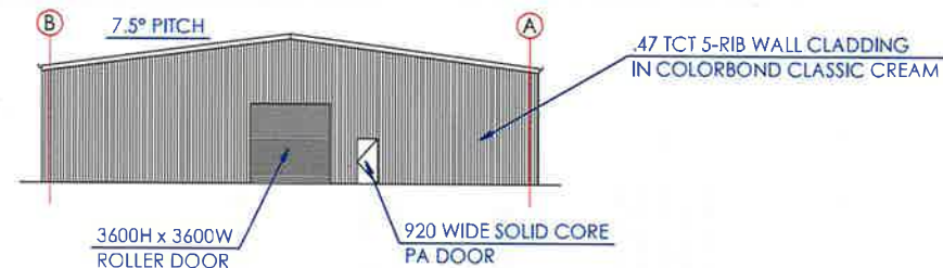
SOUTH ELEVATION
